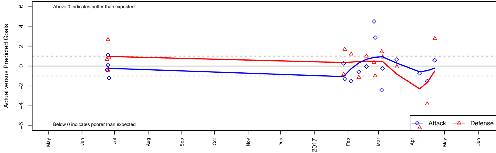
TFA Willamette Crew B02 Dots are actual minus expected GF (blue circles) and GA (red triangles). Blue line is smoothed change in attack strength. Red is smoothed change in defense strength.
